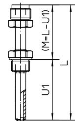
model 2 G/3 G parallel thread G1/2B G3/4B G1B M20x1,5
