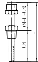
model 2 G/3 G conical thread 1/2"NPT 3/4"NPT
